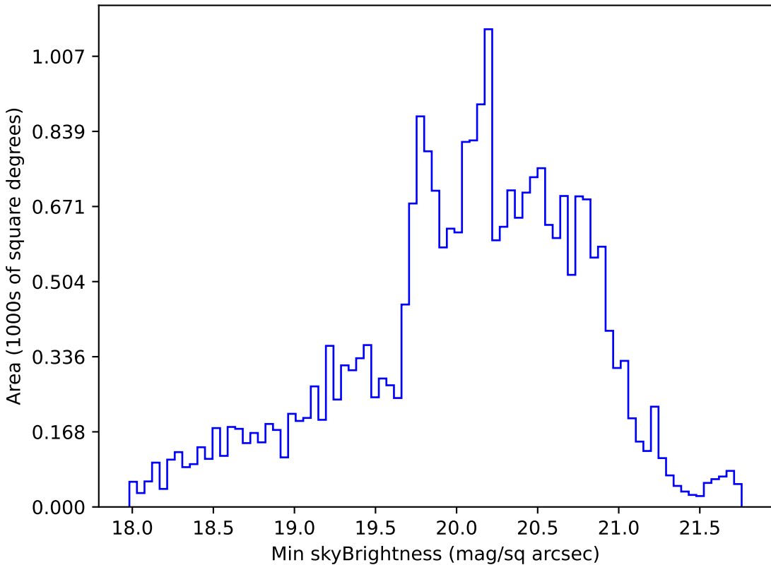
weather_cloudso18v3.4_10yrs All sky g band: Min skyBrightness
