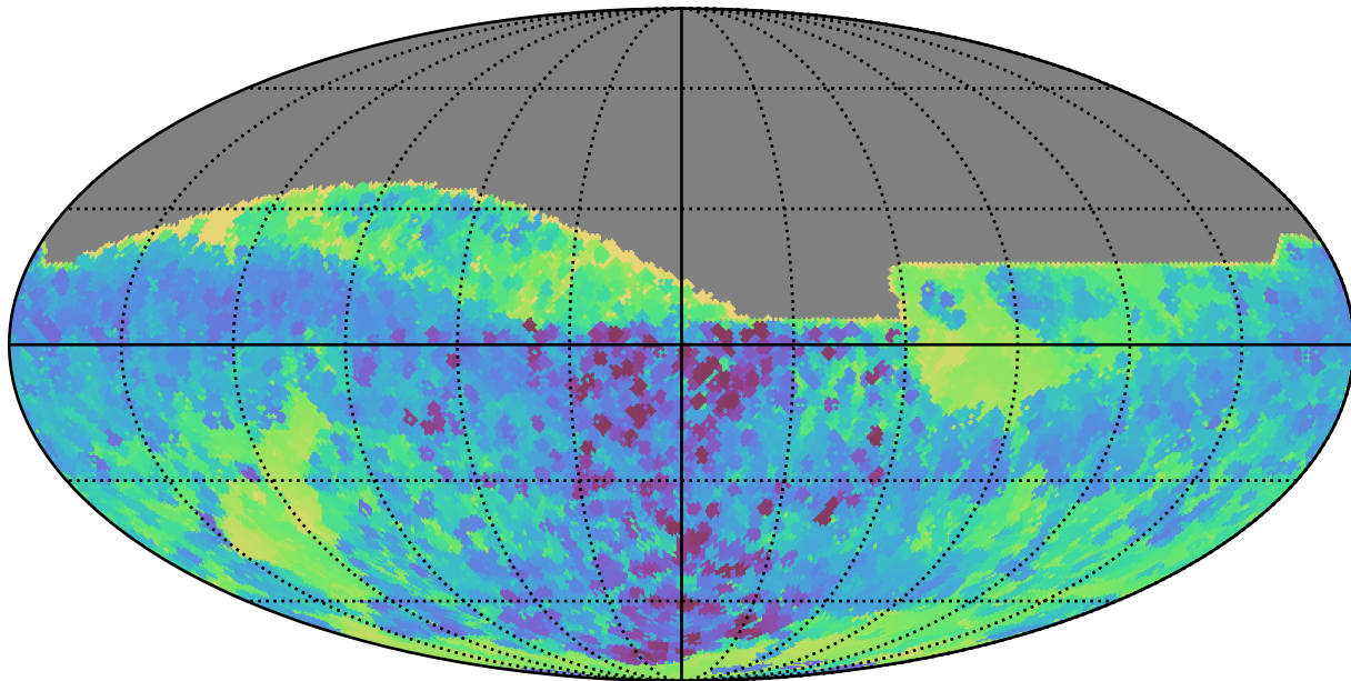
weather_cloudso18v3.4_10yrs All sky all bands: Min skyBrightness
