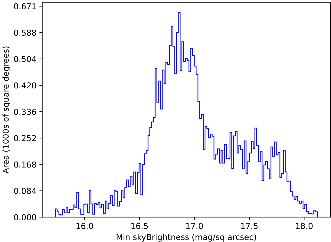
weather_cloudso18v3.4_10yrs All sky all bands: Min skyBrightness
