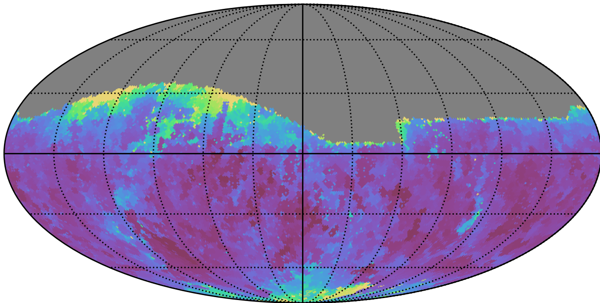
weather_cloudso18v3.4_10yrs Yr 1 r band: Min seeingEff
