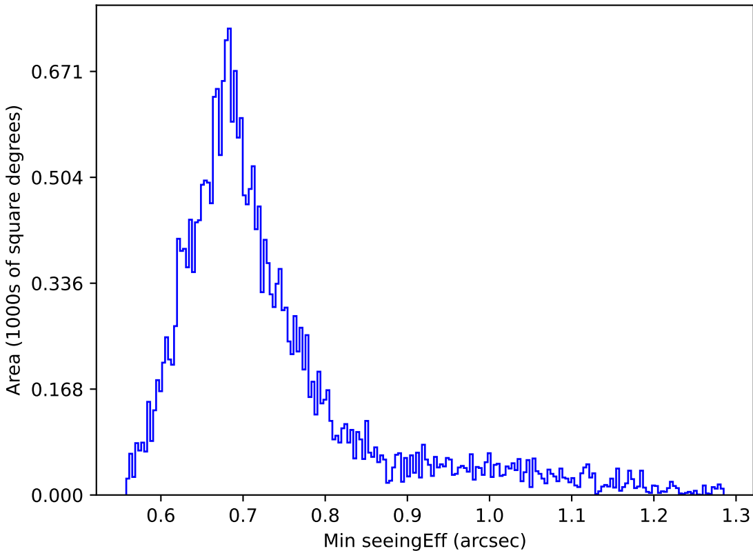
weather_cloudso18v3.4_10yrs Yr 1 i band: Min seeingEff
