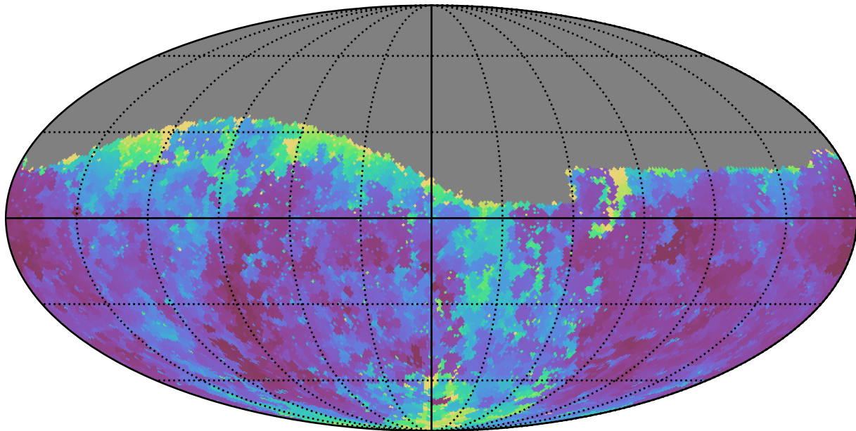
weather_cloudso18v3.4_10yrs Yr 1 g band: Min seeingEff
