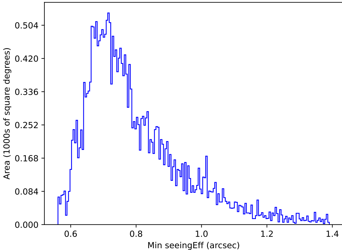
weather_cloudso18v3.4_10yrs Yr 1 g band: Min seeingEff
