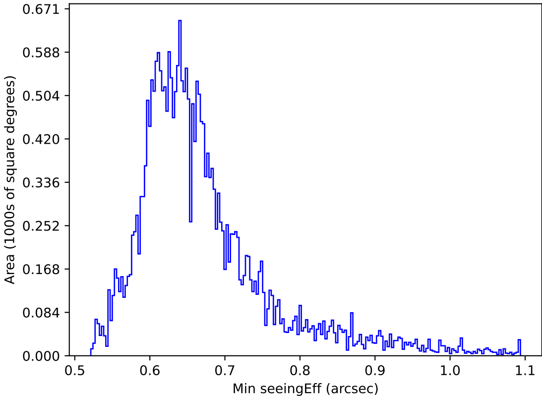
weather_cloudso18v3.4_10yrs Yr 1 all bands: Min seeingEff
