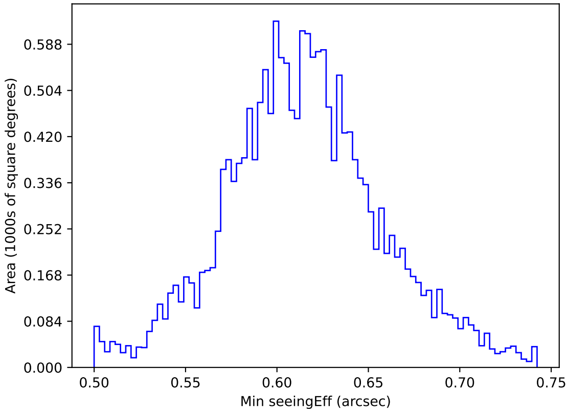
weather_cloudso18v3.4_10yrs WFD r band: Min seeingEff
