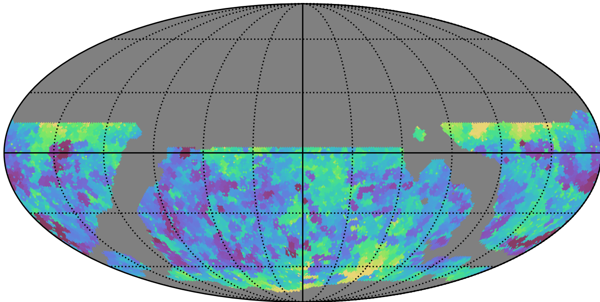
weather_cloudso18v3.4_10yrs WFD g band: Min seeingEff
