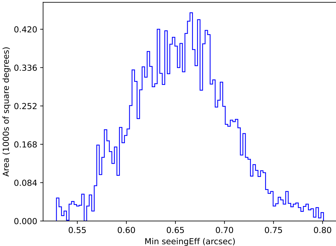
weather_cloudso18v3.4_10yrs WFD g band: Min seeingEff
