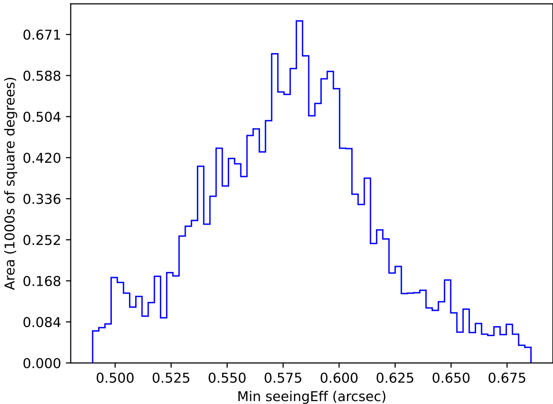
weather_cloudso18v3.4_10yrs WFD all bands: Min seeingEff
