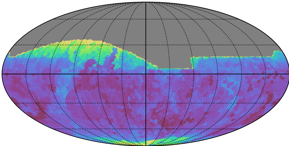
weather_cloudso18v3.4_10yrs All sky z band: Min seeingEff
