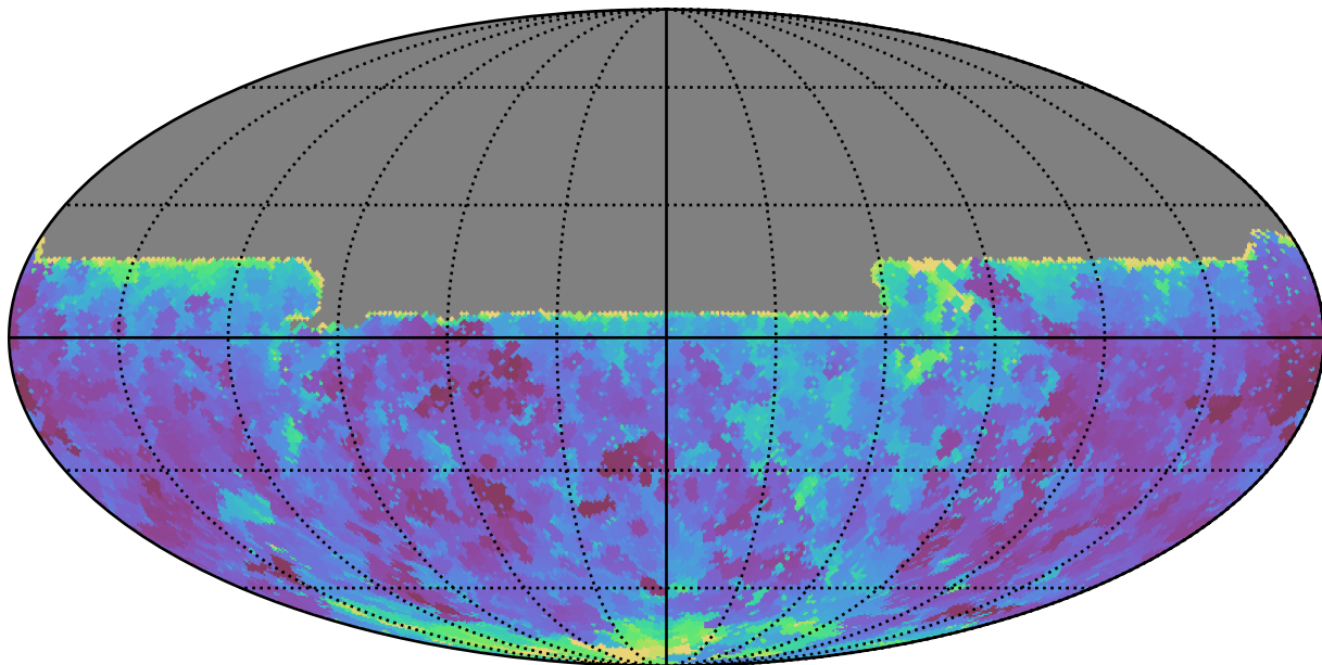
weather_cloudso18v3.4_10yrs All sky u band: Min seeingEff
