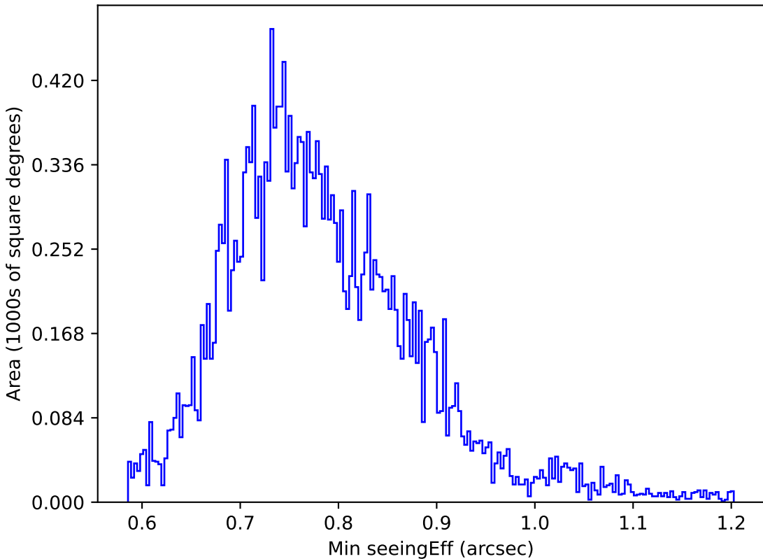
weather_cloudso18v3.4_10yrs All sky u band: Min seeingEff
