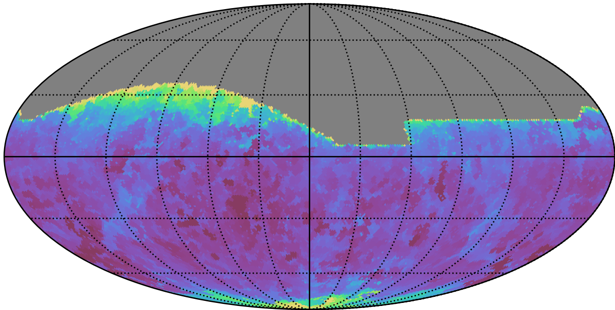
weather_cloudso18v3.4_10yrs All sky r band: Min seeingEff
