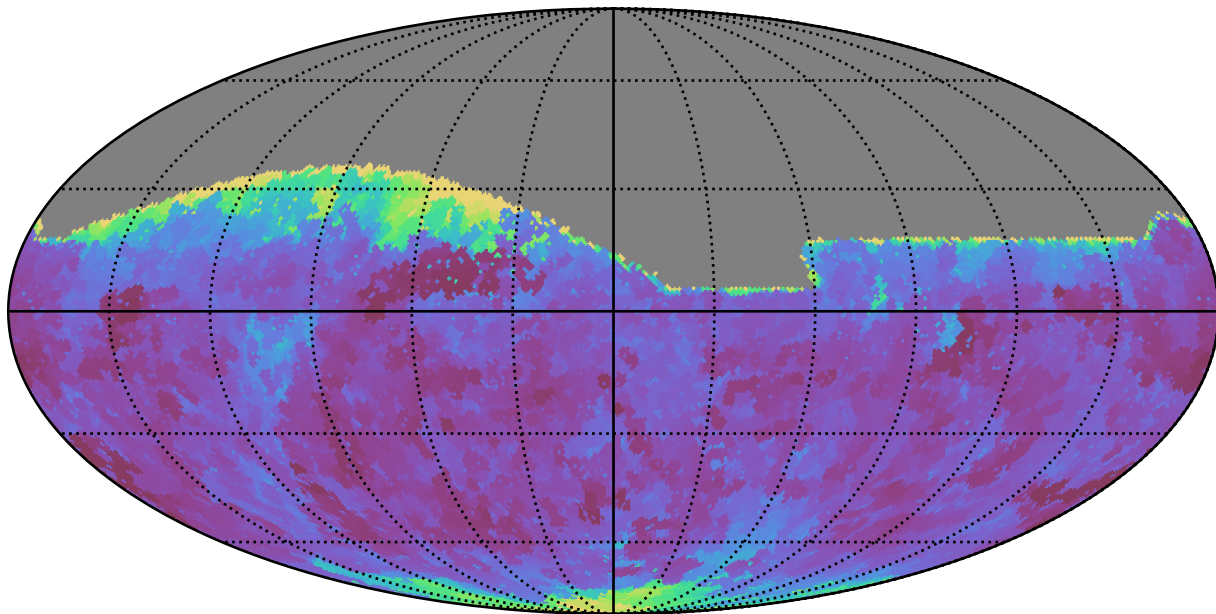
weather_cloudso18v3.4_10yrs All sky g band: Min seeingEff
