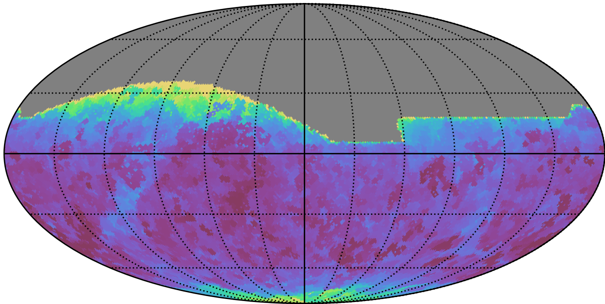
weather_cloudso18v3.4_10yrs All sky all bands: Min seeingEff
