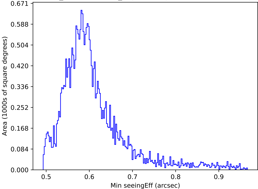
weather_cloudso18v3.4_10yrs All sky all bands: Min seeingEff
