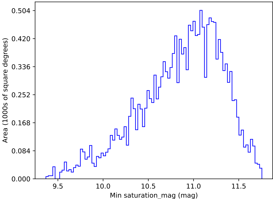
weather_cloudso18v3.4_10yrs WFD all bands: Min saturation_mag
