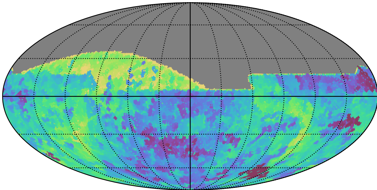
weather_cloudso18v3.4_10yrs All sky all bands: Min saturation_mag
