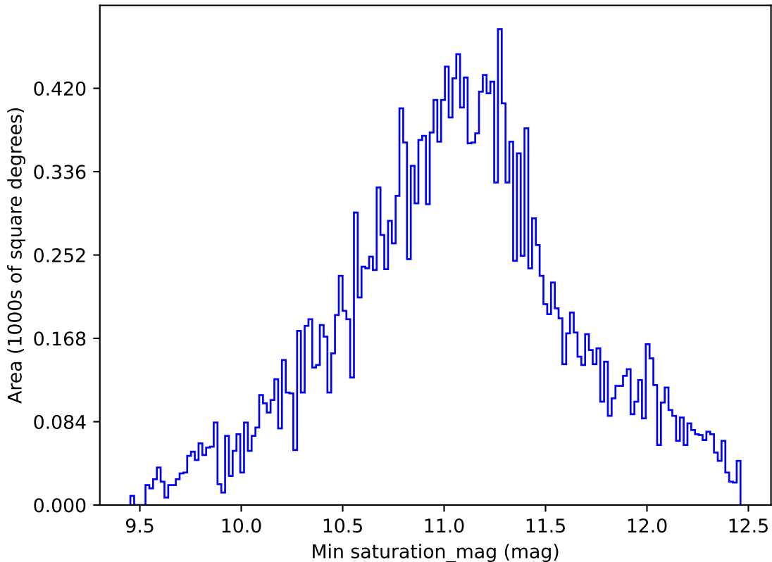
weather_cloudso18v3.4_10yrs All sky all bands: Min saturation_mag
