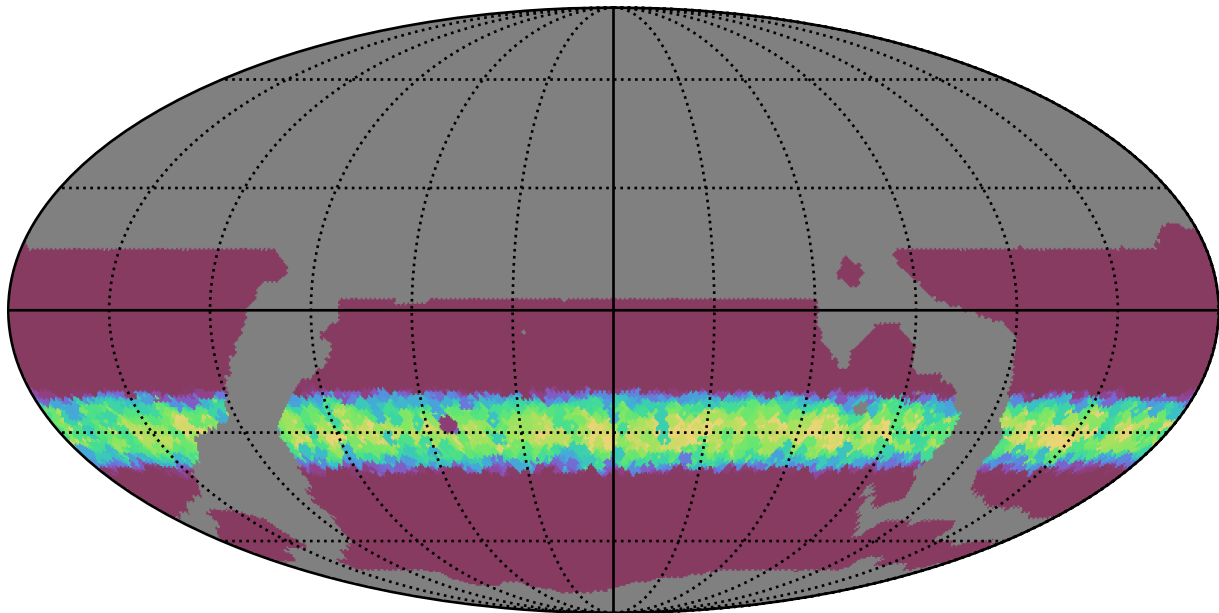
weather_cloudso18v3.4_10yrs WFD all bands: Min normairmass
