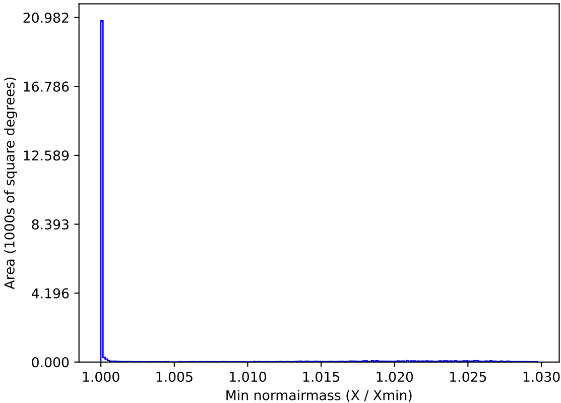
weather_cloudso18v3.4_10yrs All sky all bands: Min normairmass
