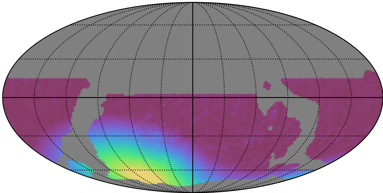
weather_cloudso18v3.4_10yrs WFD z band: Min moonDistance
