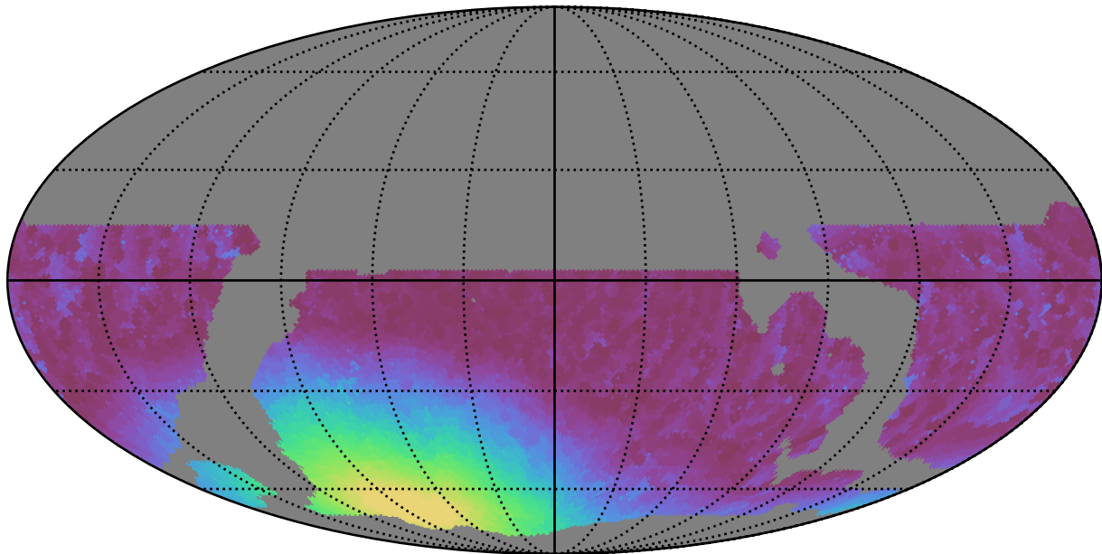
weather_cloudso18v3.4_10yrs WFD r band: Min moonDistance
