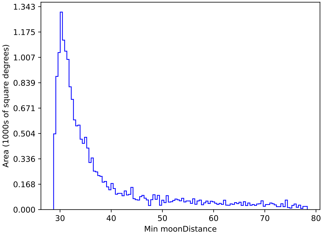
weather_cloudso18v3.4_10yrs WFD r band: Min moonDistance
