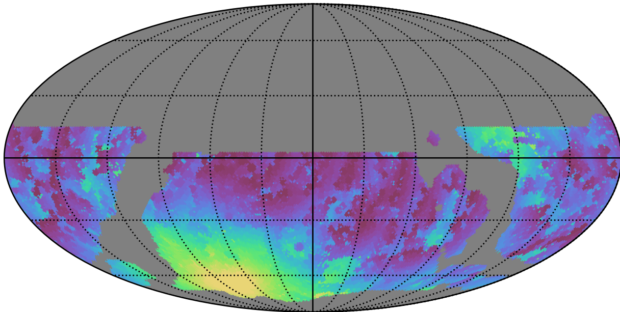
weather_cloudso18v3.4_10yrs WFD g band: Min moonDistance
