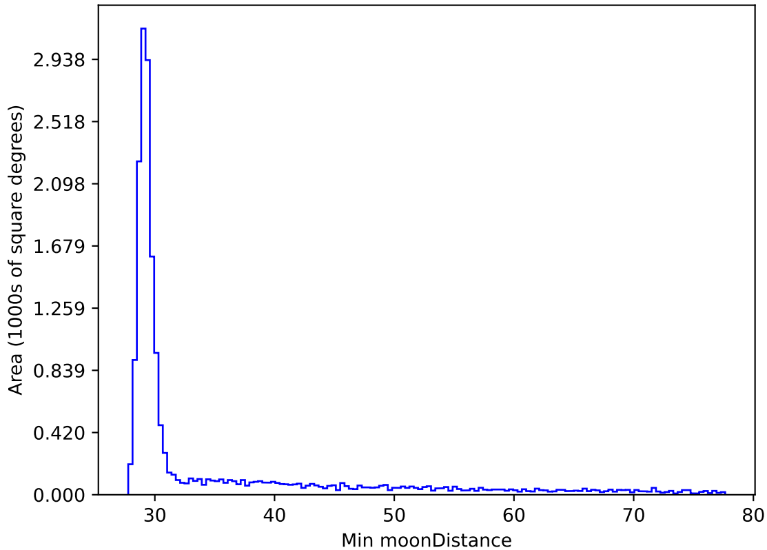
weather_cloudso18v3.4_10yrs WFD all bands: Min moonDistance
