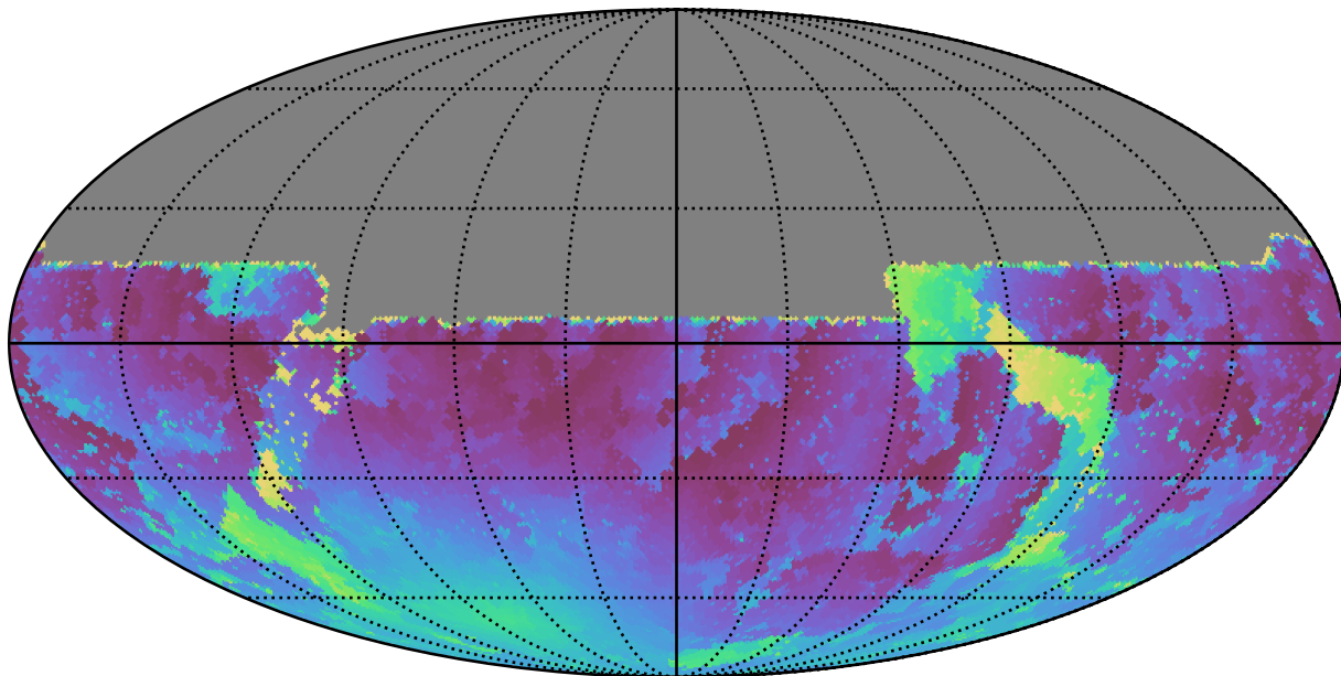
weather_cloudso18v3.4_10yrs All sky u band: Min moonDistance
