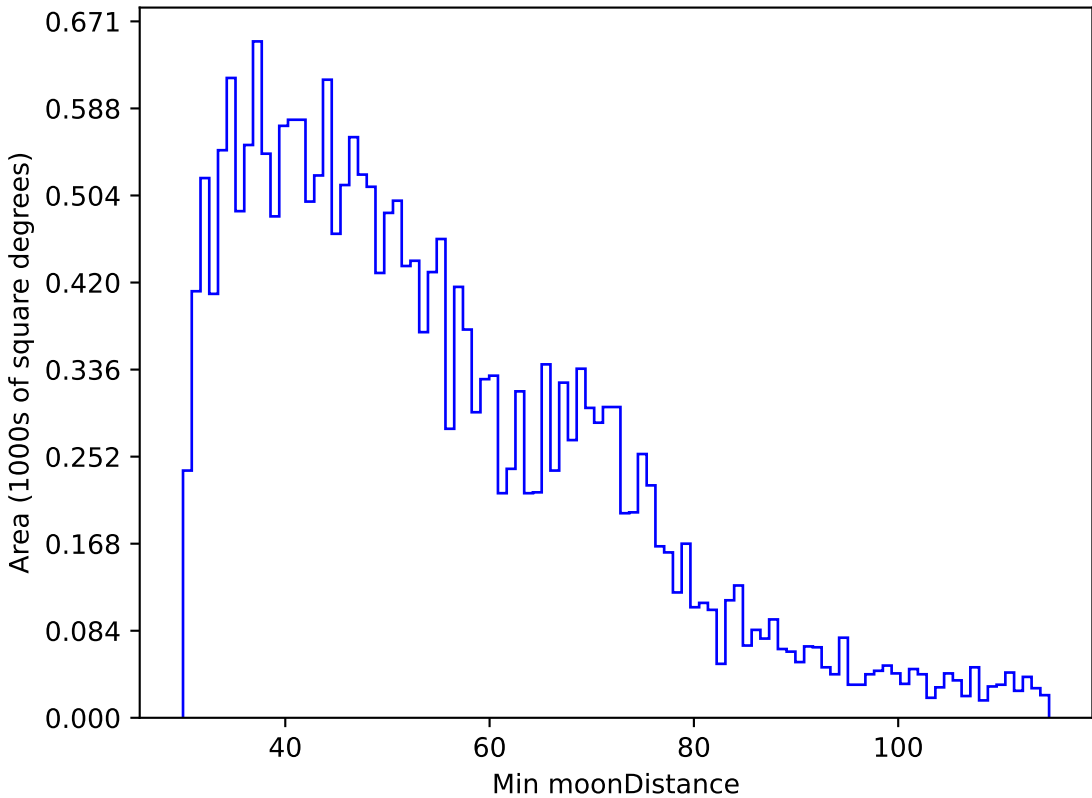
weather_cloudso18v3.4_10yrs All sky u band: Min moonDistance
