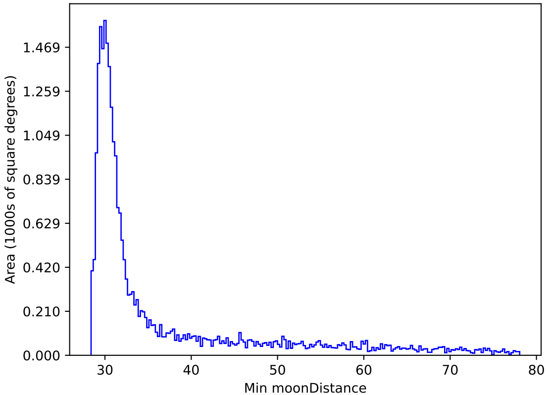
weather_cloudso18v3.4_10yrs All sky i band: Min moonDistance
