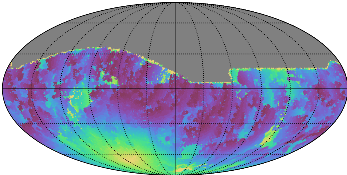
weather_cloudso18v3.4_10yrs All sky g band: Min moonDistance
