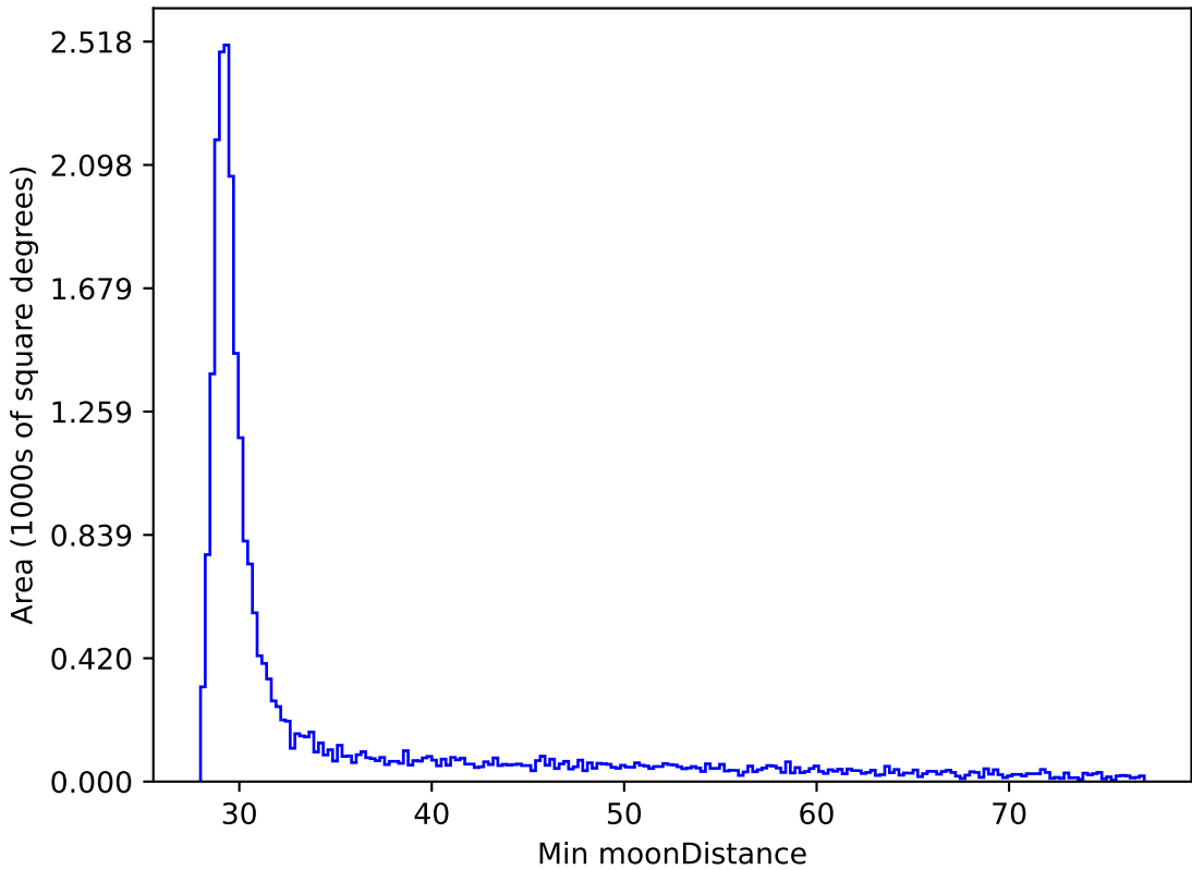
weather_cloudso18v3.4_10yrs All sky all bands: Min moonDistance
