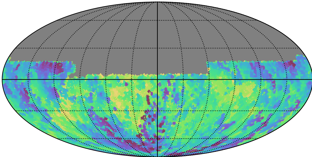
weather_cloudso18v3.4_10yrs Yr 1 y band: Min fiveSigmaDepth
