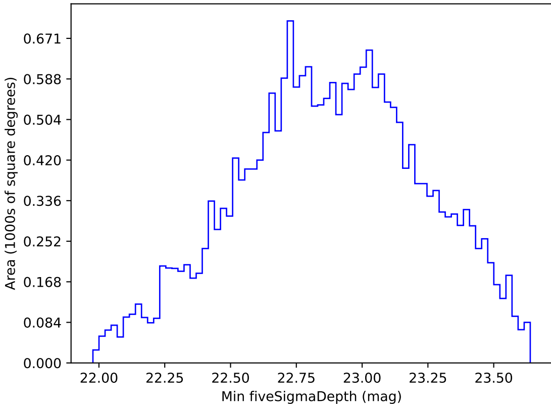
weather_cloudso18v3.4_10yrs Yr 1 u band: Min fiveSigmaDepth
