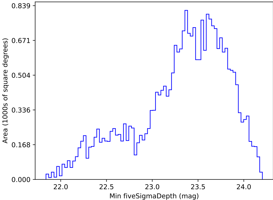
weather_cloudso18v3.4_10yrs Yr 1 r band: Min fiveSigmaDepth
