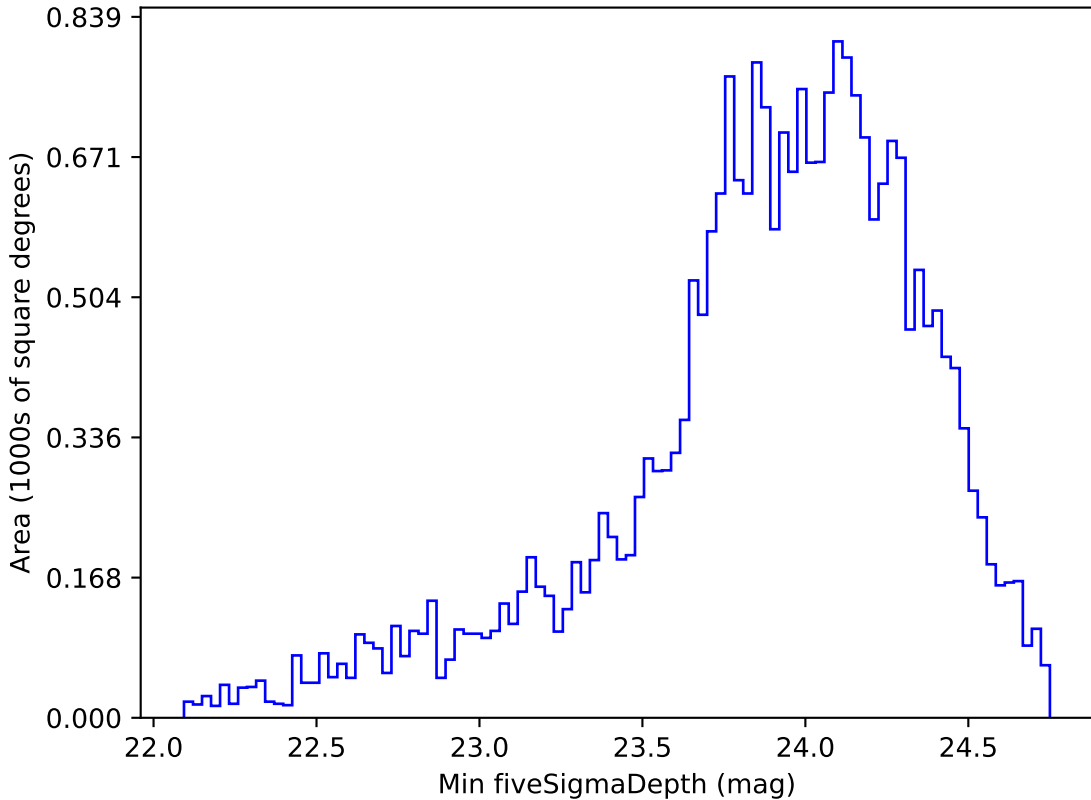
weather_cloudso18v3.4_10yrs Yr 1 g band: Min fiveSigmaDepth
