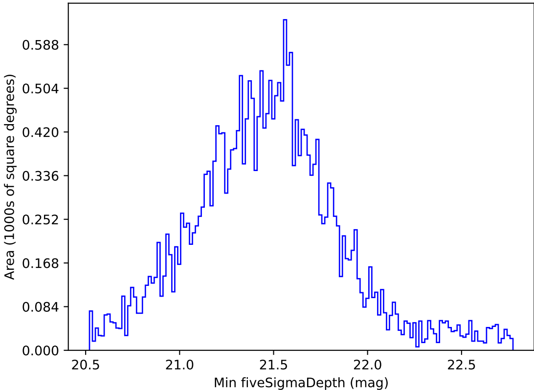
weather_cloudso18v3.4_10yrs Yr 1 all bands: Min fiveSigmaDepth
