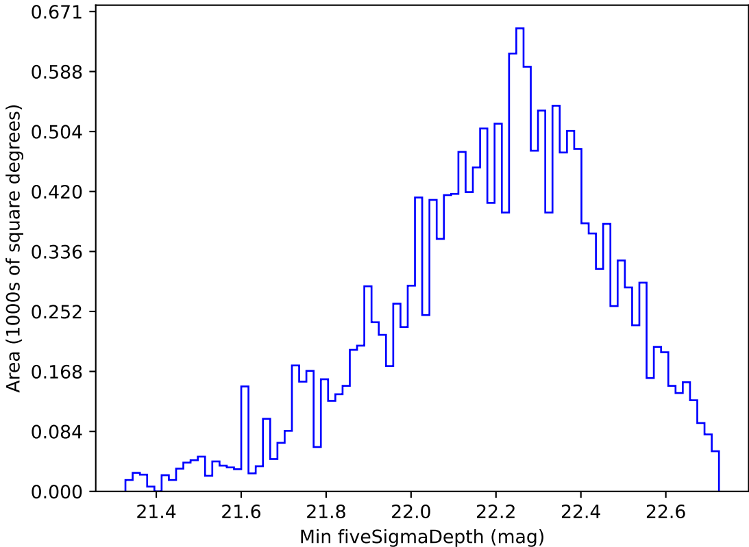
weather_cloudso18v3.4_10yrs WFD u band: Min fiveSigmaDepth
