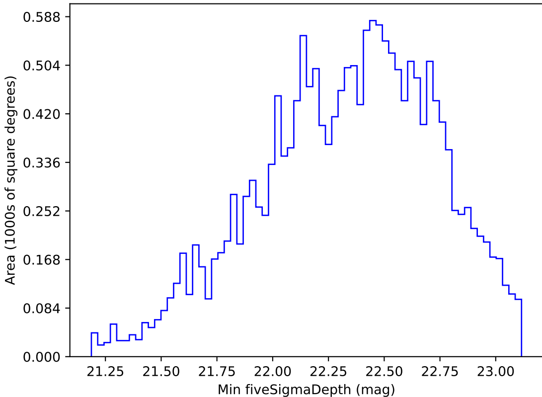
weather_cloudso18v3.4_10yrs WFD r band: Min fiveSigmaDepth
