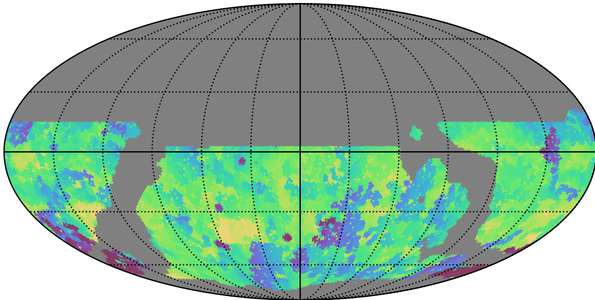
weather_cloudso18v3.4_10yrs WFD g band: Min fiveSigmaDepth
