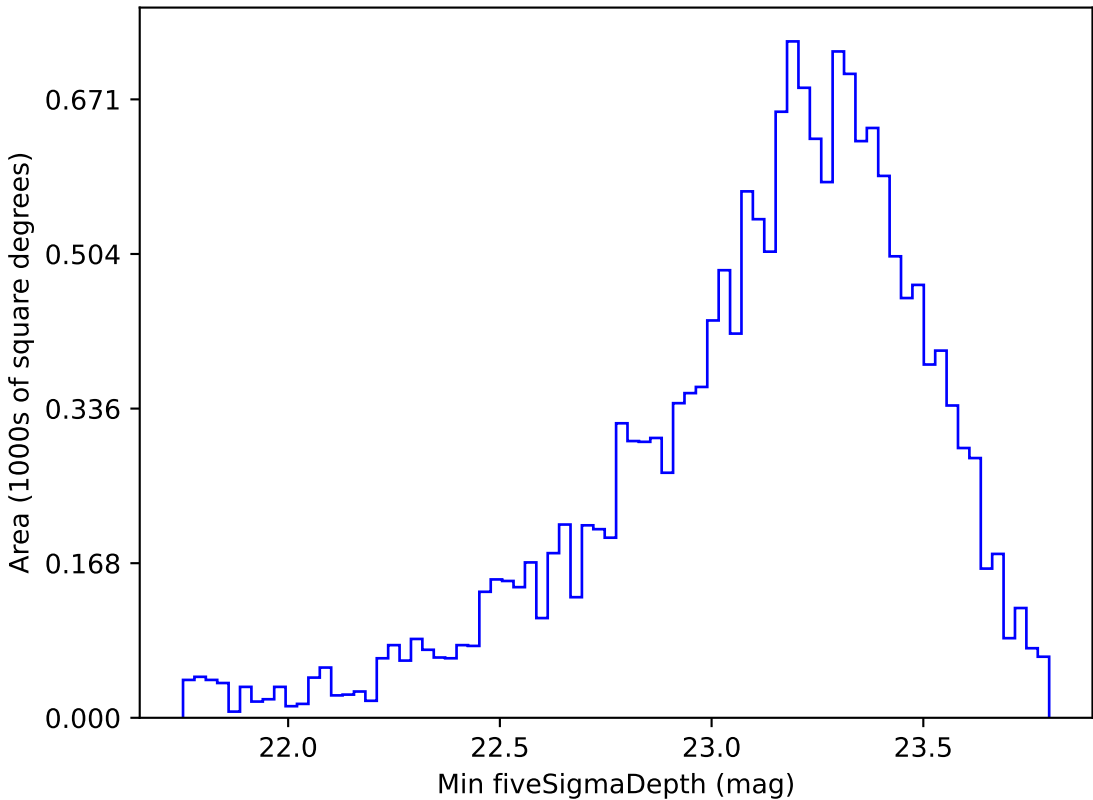
weather_cloudso18v3.4_10yrs WFD g band: Min fiveSigmaDepth
