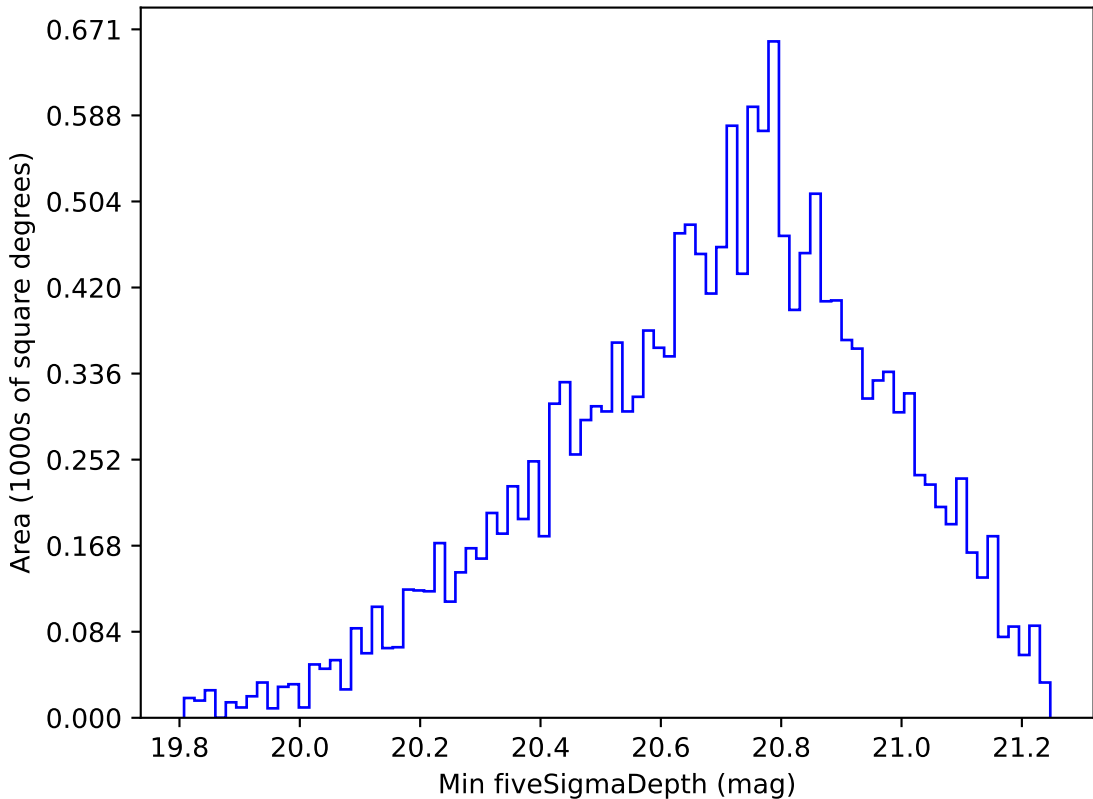
weather_cloudso18v3.4_10yrs WFD all bands: Min fiveSigmaDepth
