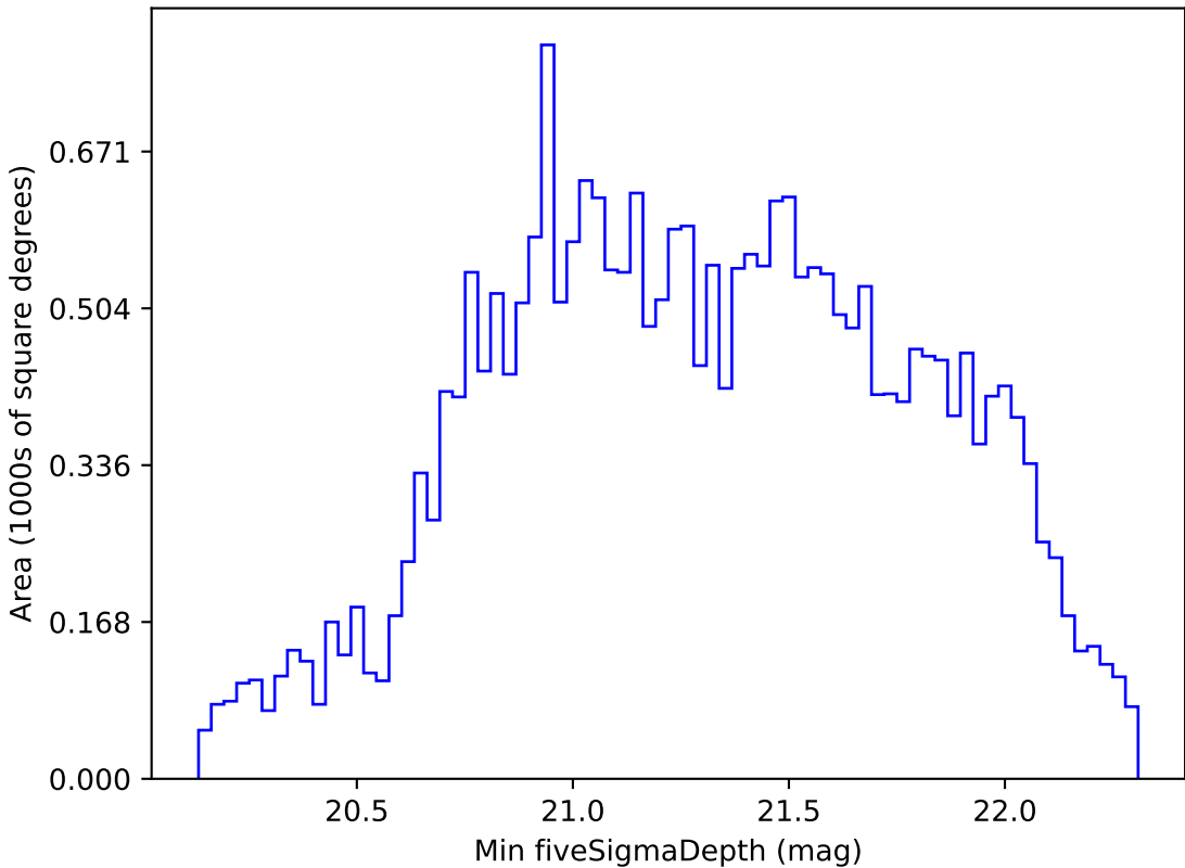
weather_cloudso18v3.4_10yrs All sky z band: Min fiveSigmaDepth
