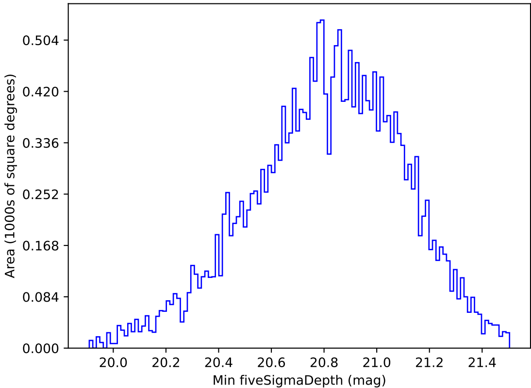
weather_cloudso18v3.4_10yrs All sky y band: Min fiveSigmaDepth
