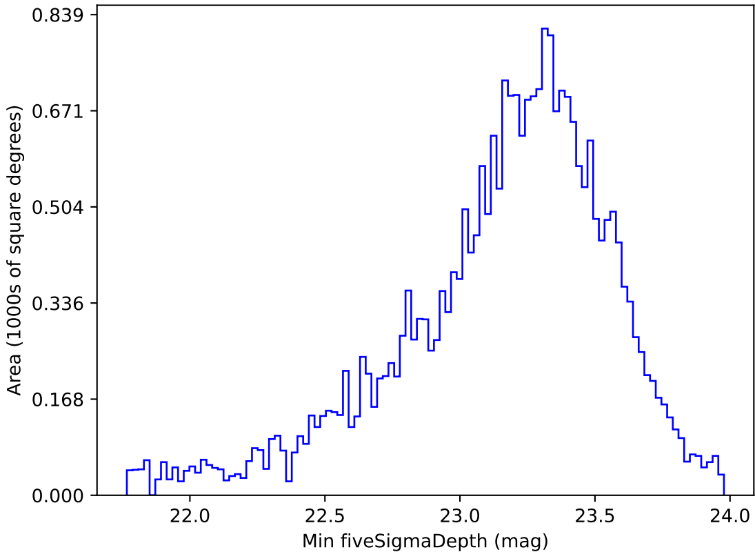
weather_cloudso18v3.4_10yrs All sky g band: Min fiveSigmaDepth
