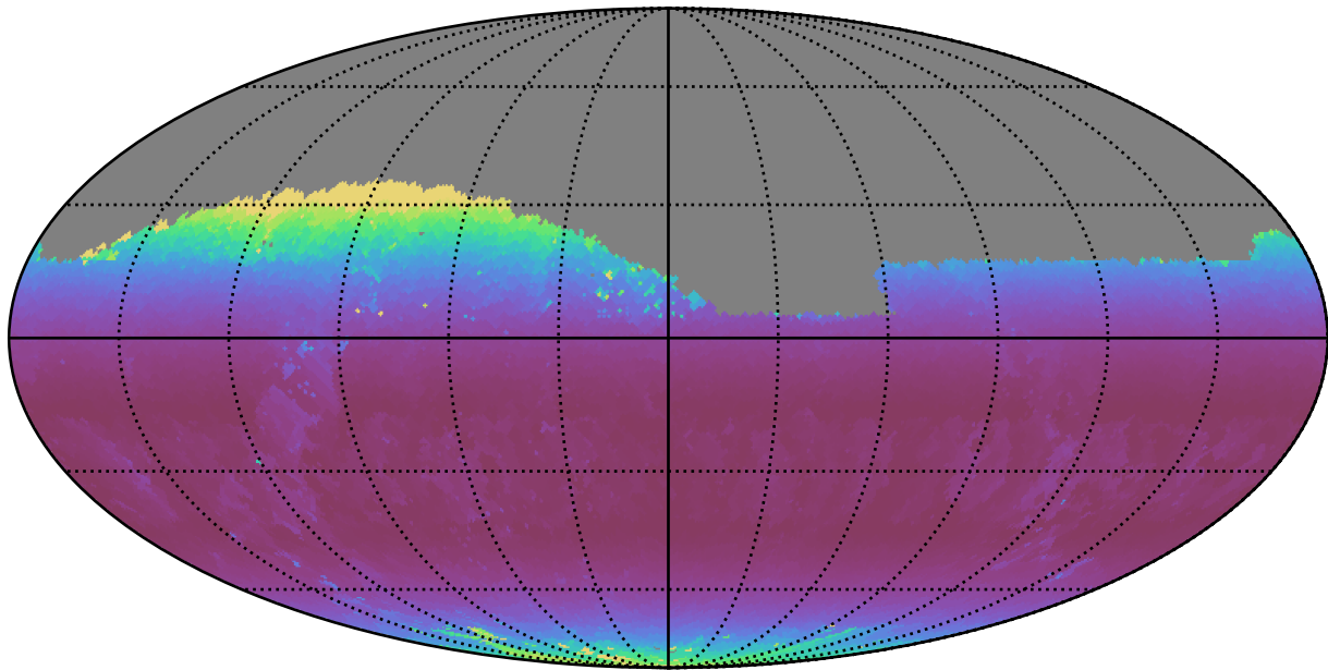
weather_cloudso18v3.4_10yrs Yr 1 z band: Min airmass
