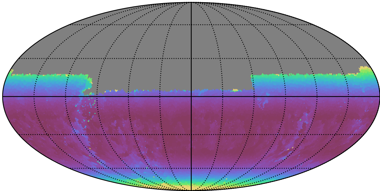
weather_cloudso18v3.4_10yrs Yr 1 y band: Min airmass
