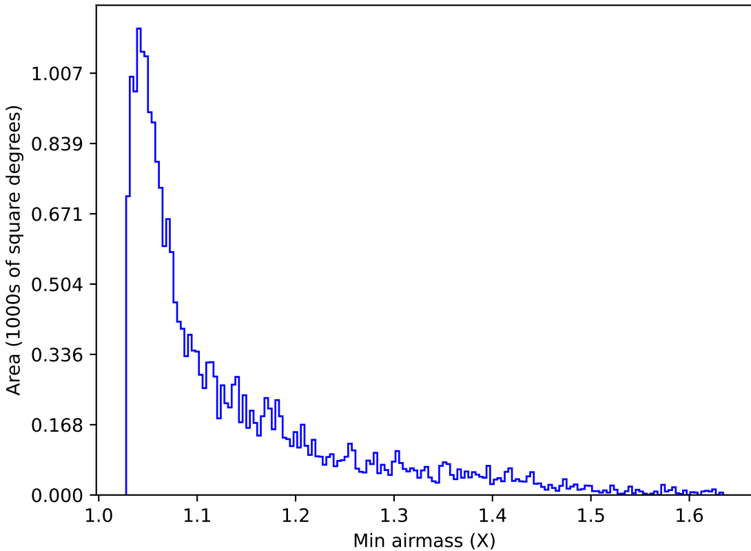
weather_cloudso18v3.4_10yrs Yr 1 y band: Min airmass
